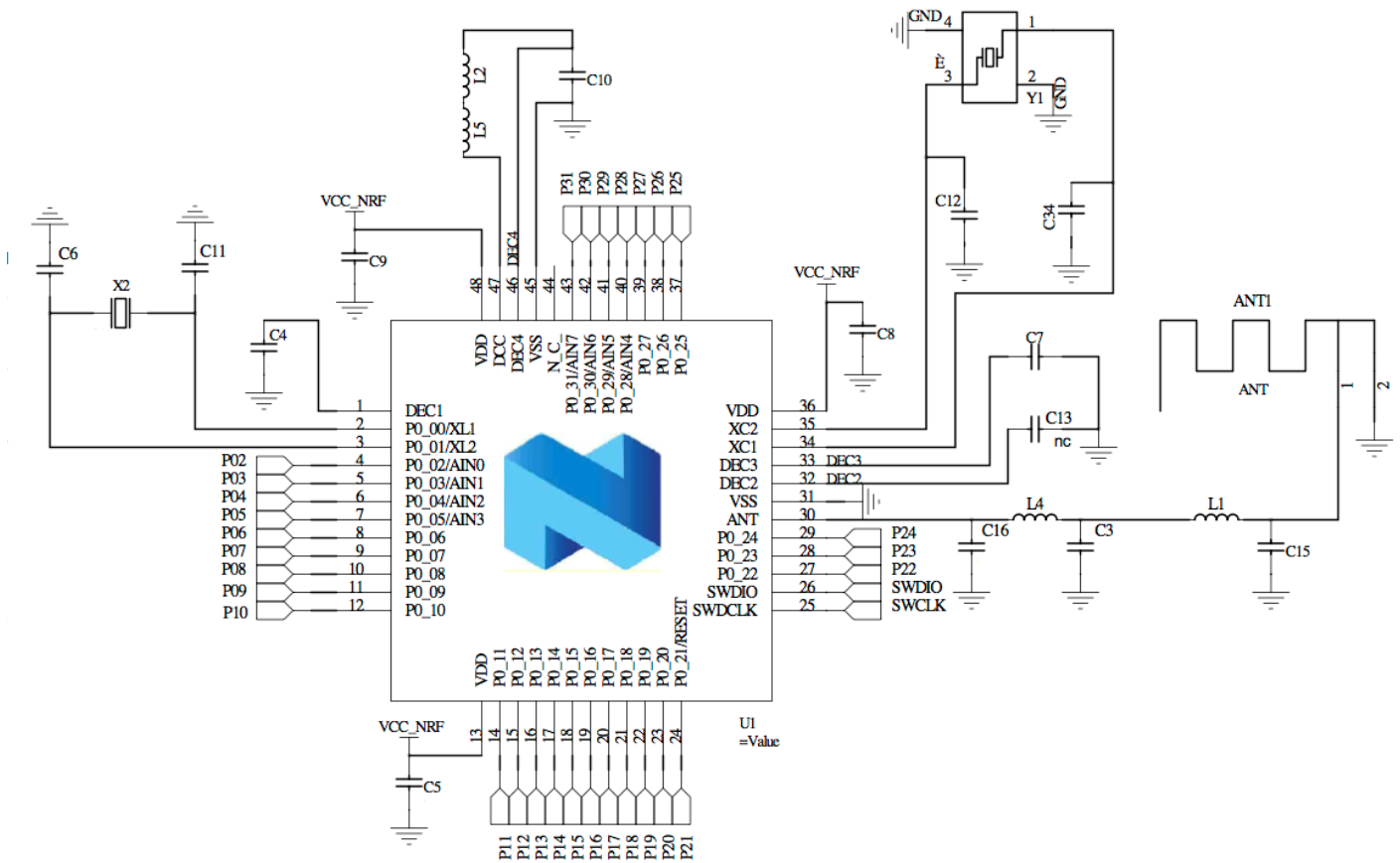
Figure 6. Schematic Diagram of RF-BM-ND08C
