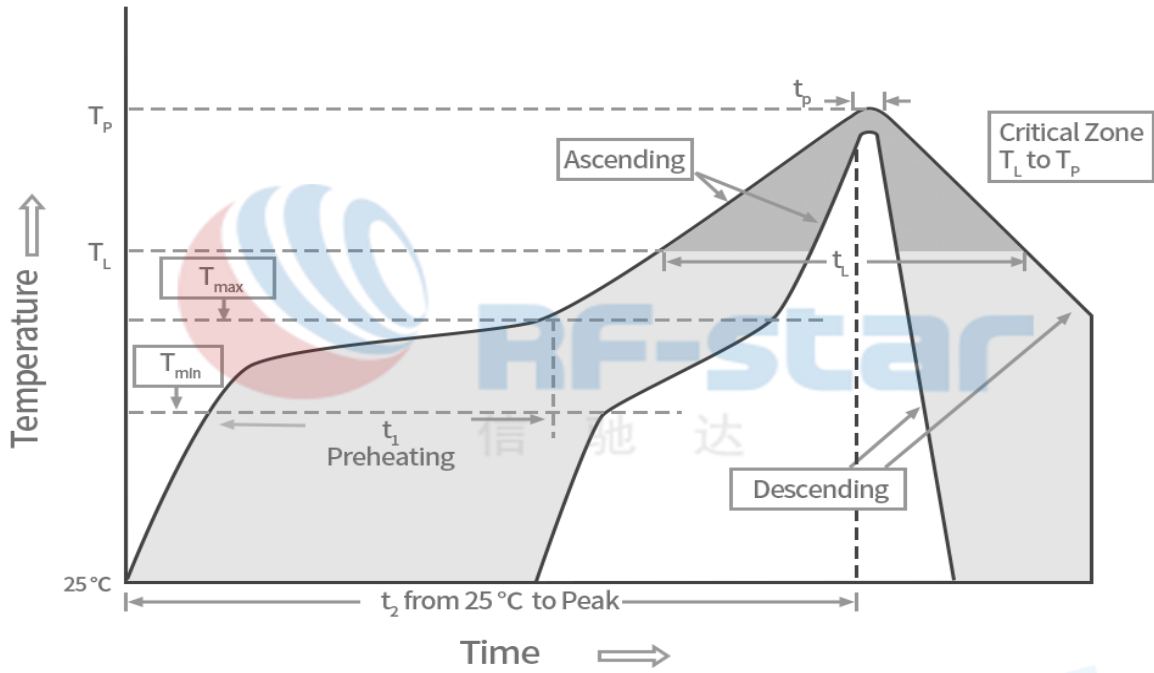
Figure 13. Recommended Reflow for Lead-Free Solder
