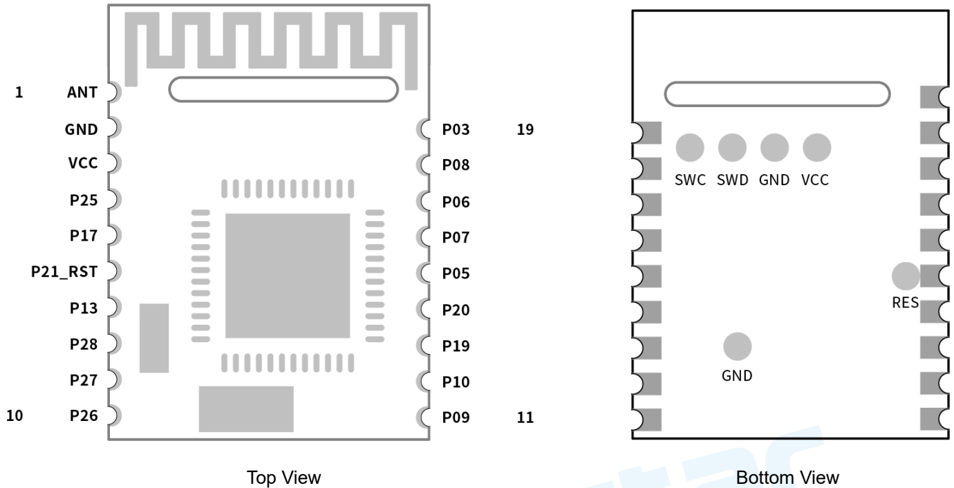
Figure 3. Pin Diagram of RF-BM-ND08C
