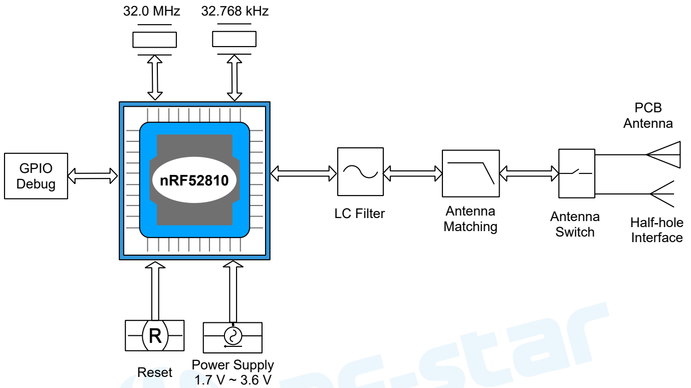
Figure 1. Functional Block Diagram of RF-BM-ND08C
