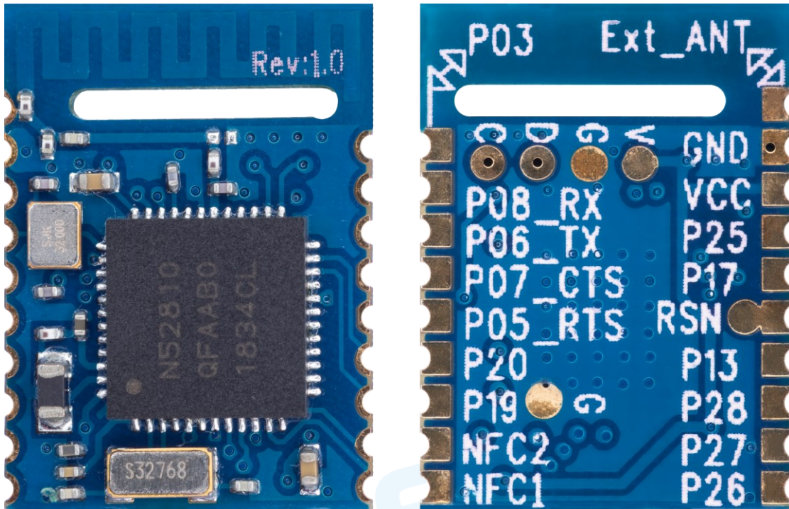
Figure 4. Photos of RF-BM-ND08C
