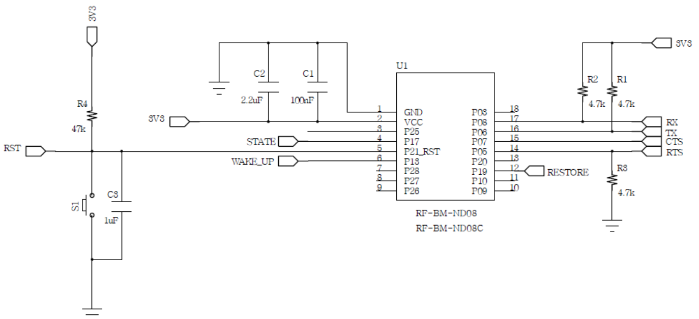
Figure 7. Reference Design of RF-BM-ND08C
