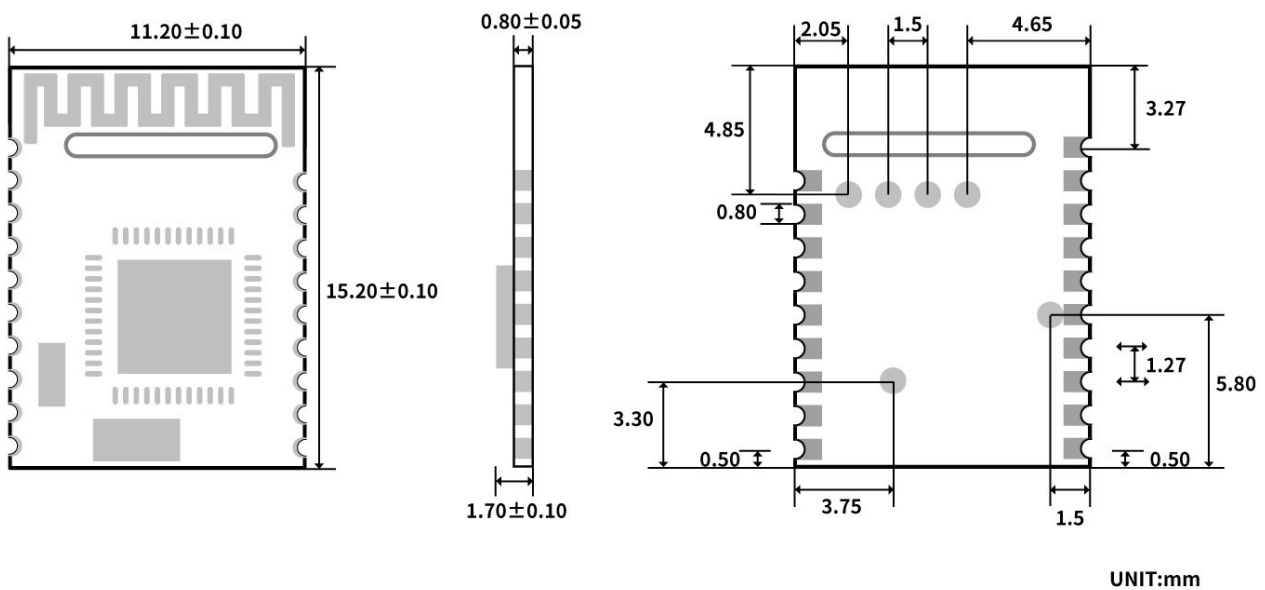
Figure 5. Recommended PCB Footprint of RF-BM-ND08C (mm)
