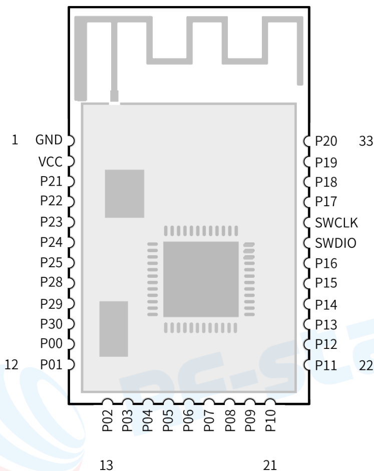
Figure 3. Pin Diagram of RF-BM-ND01
