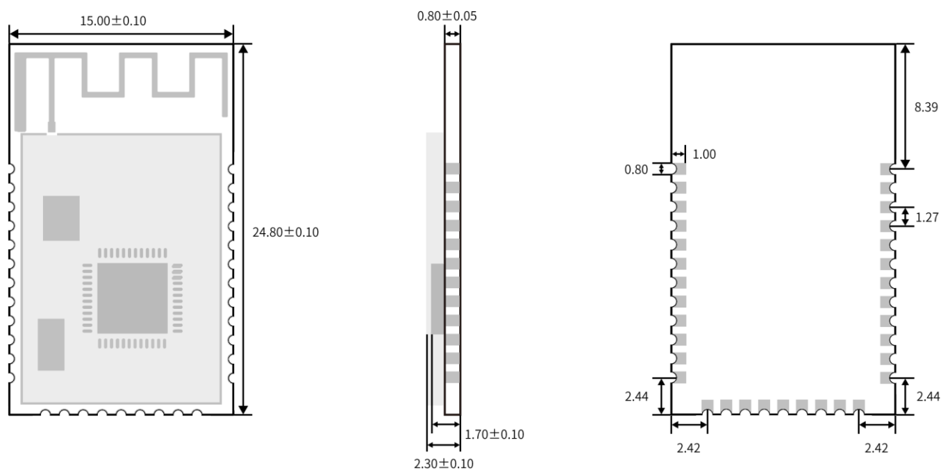
Figure 5. Recommended PCB Footprint of RF-BM-ND01 (mm)
