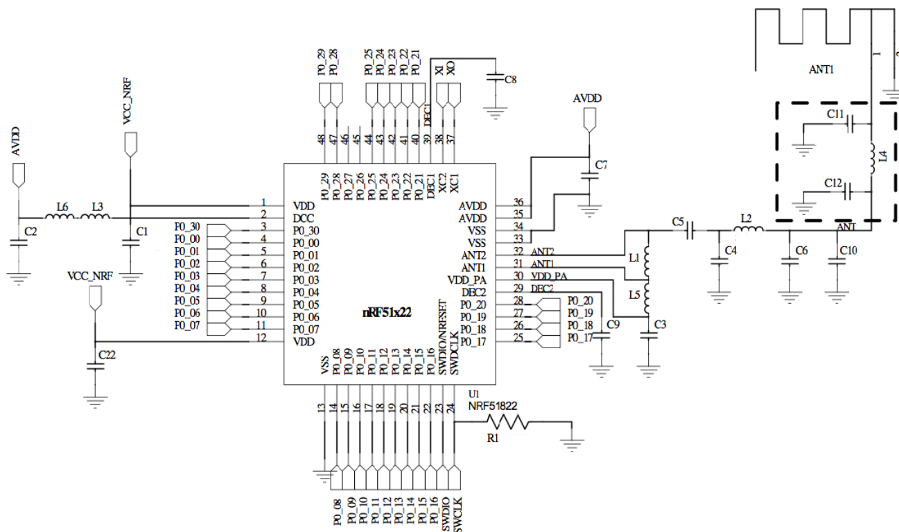
Figure 6. Schematic Diagram of RF-BM-ND01
