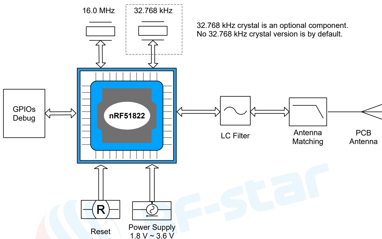
Figure 1. Functional Block Diagram of RF-BM-ND01
