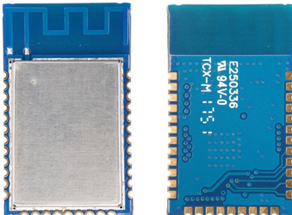
Figure 4. Photos of RF-BM-ND01
