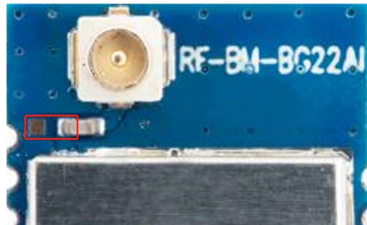
Figure 9. Antenna Output Mode Change of RF-BM-BG22A1I
