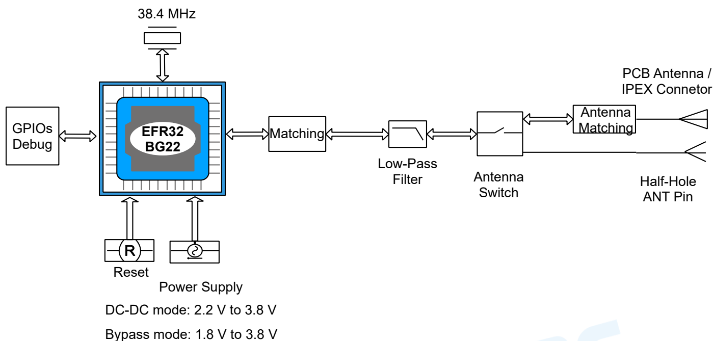
Figure 1. Functional Block Diagram of RF-BM-BG22A3(I)
