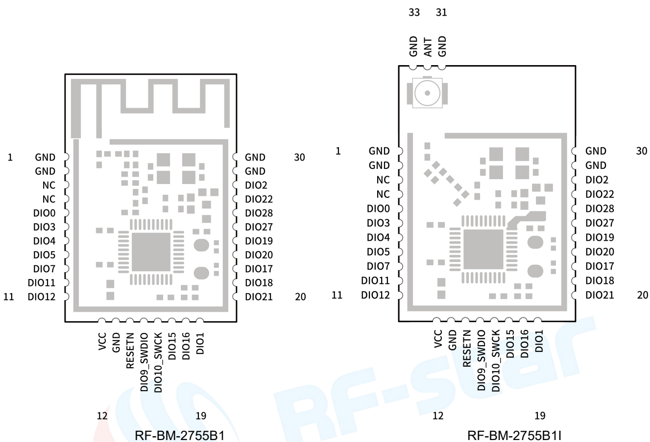
Figure 3. Pin Diagram of RF-BM-2755B1(I)
