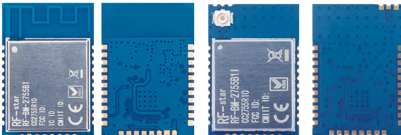
RF-BM-2755B1
