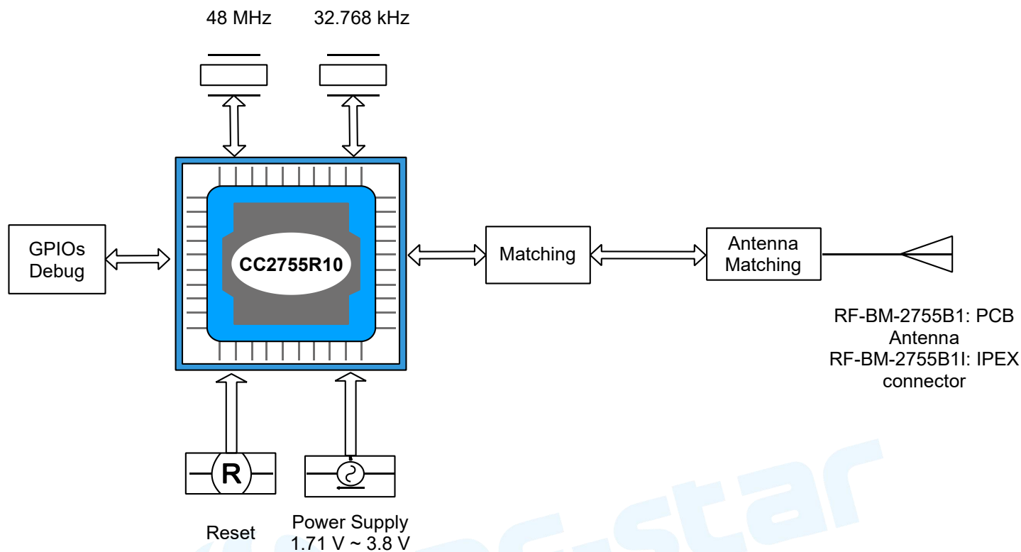
Figure 1. Functional Block Diagram of RF-BM-2755B1(I)
