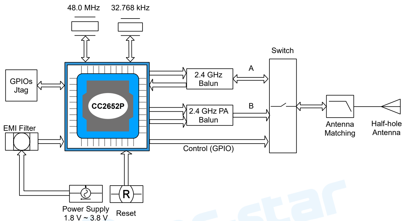
Figure 1. Functional Block Diagram of RF-BM-2652P1
