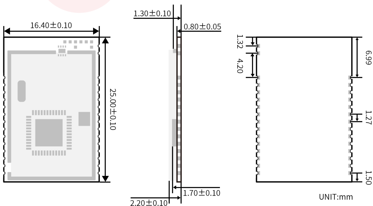
Figure 4. Recommended PCB Footprint of RF-BM-2652P1
