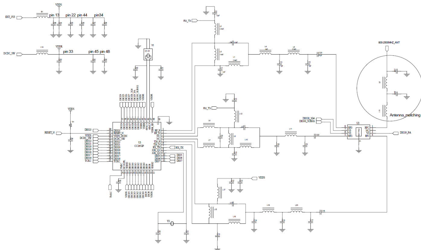
Figure 5. Schematic Diagram of RF-BM-2652P1
