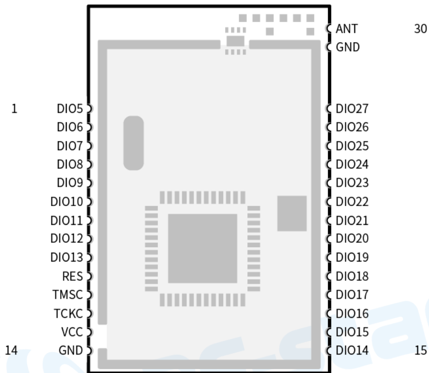
Figure 3. Pin Diagram of RF-BM-2652P1
