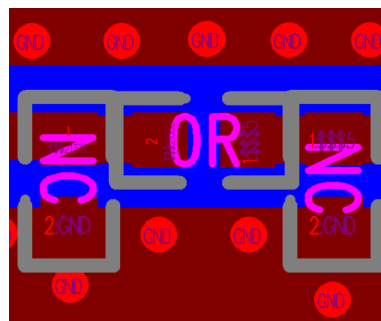
Figure 6. Reference Design of the External Antenna Traces
