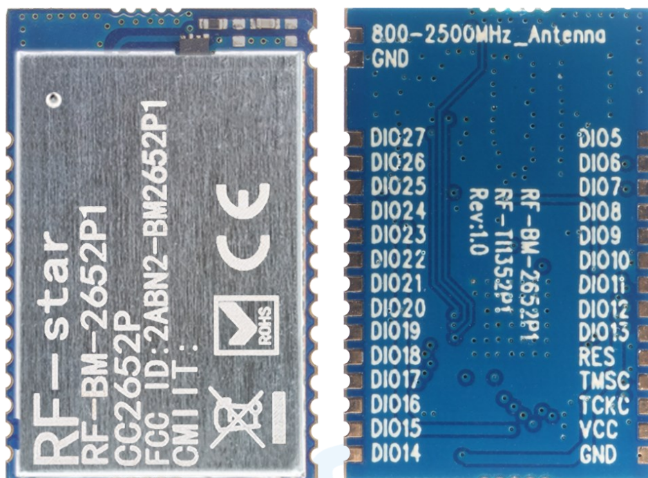
Figure 3. Photos of RF-BM-2652P1
