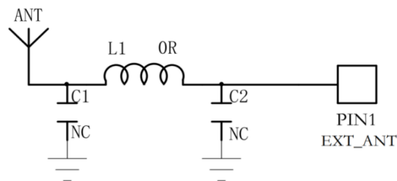
Figure 5. Reference Design of the External Antenna
