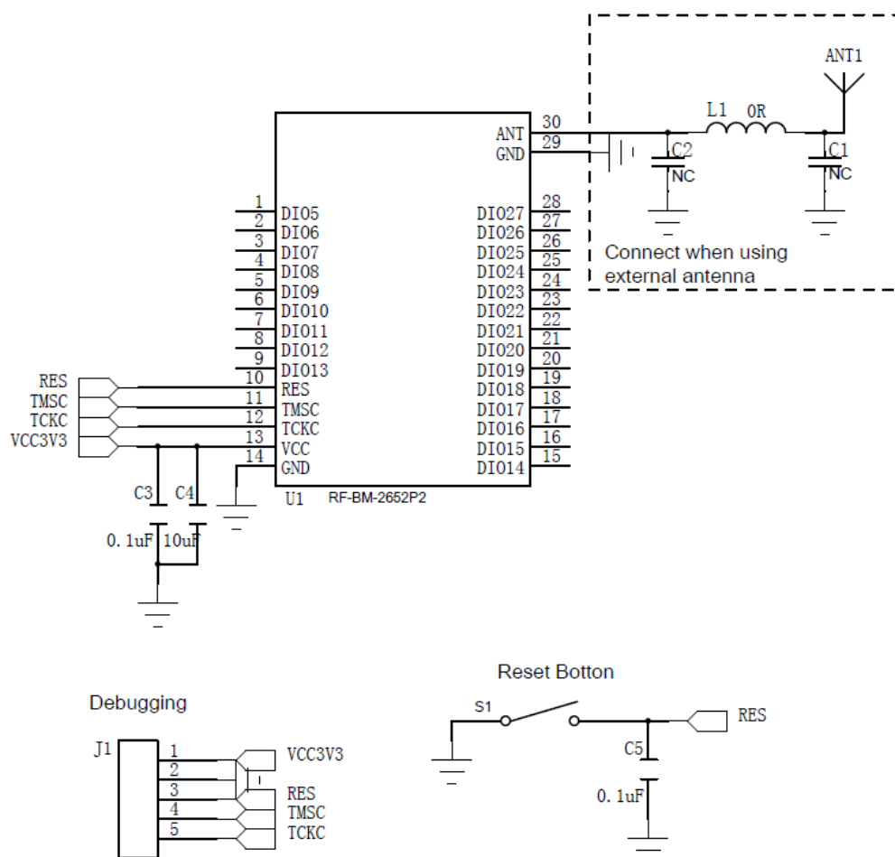
Figure 5. Reference Design of RF-BM-2652P1
